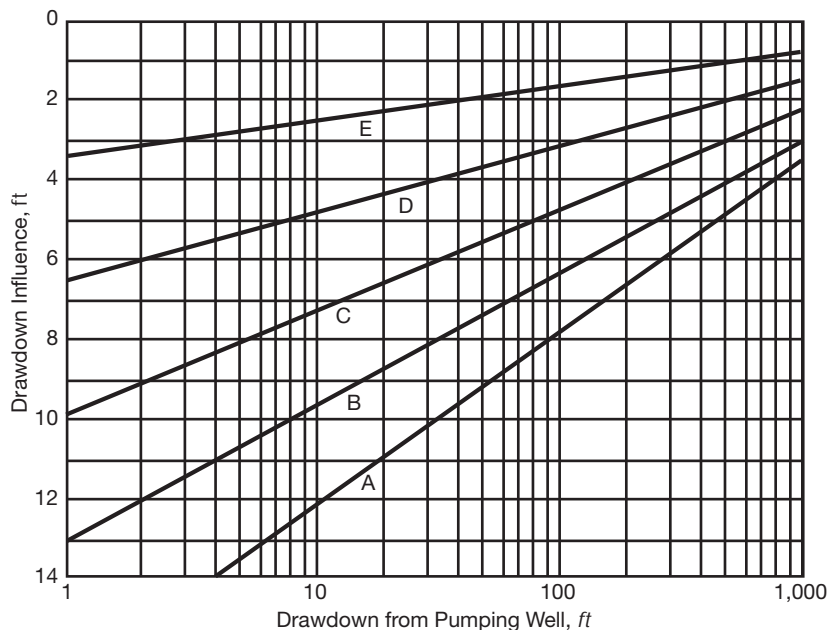
Figure 5-32 Influence for various rates of pumping in an aquifer
