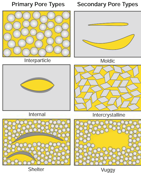
Fig. 1.2 Diagrams of common pore type (yellow) in sedimentary rock. Primary pores are present in unaltered sediments. Secondary pores form after deposition as the result of dissolution and replacement processes. Secondary pores may form the dissolution of single grains (moldic) or may be much larger than the size of grains (vuggy)
