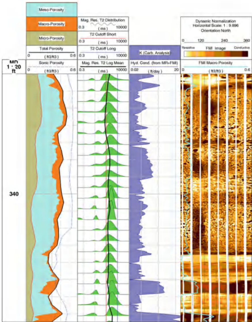
Fig. 10.14 NMR and FMI log from an ASR exploratory well in Florida. Bedding and small vugs caused by the dissolution of fossils are evident in the FMI log (right track). The T2 distributions (second track from left) and FMI macroporosity are used to determine the pore-size distribution (left) track and hydraulic conductivity (third track from left)
