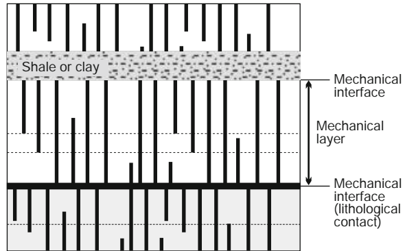
Fig. 17.5 Mechanical integrity concepts. Fractures (black) terminate at mechanical interfaces, such as shale (or clay) beds and other lithological contacts, which may be the location of horizontal fractures. Mechanical interfaces bound mechanical units (layers)
