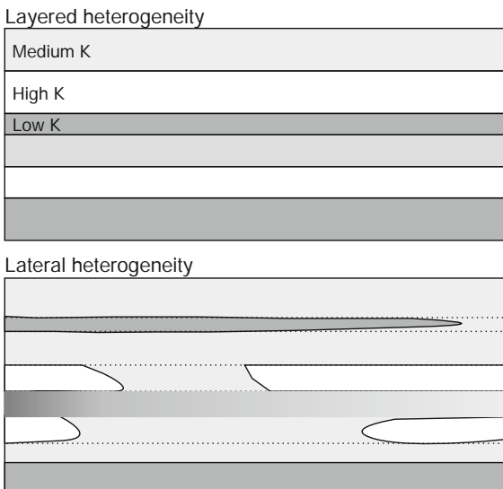
Fig. 1.3 Conceptual diagram of layered and lateral heterogeneity. Lateral heterogeneity may be due to discontinuities of sediment bodies or more gradual changes in properties with an aquifer layer. The data requirements to characterize lateral heterogeneity are much greater than that needed for layered heterogeneity
