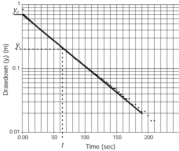
Fig. 8.5 Semilog plot of slug test data from Daytona Beach, Florida, illustrating the graphical determination of the y_0 , y_t , and t parameters for the Bouwer and Rice (1976) method
