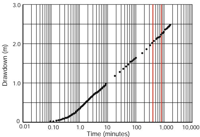
Fig. 7.1 Semilog time-drawdown plot. A doubling of the test duration from 400 to 800 min (red lines) results in a comparatively much shorter increase in the plot length
