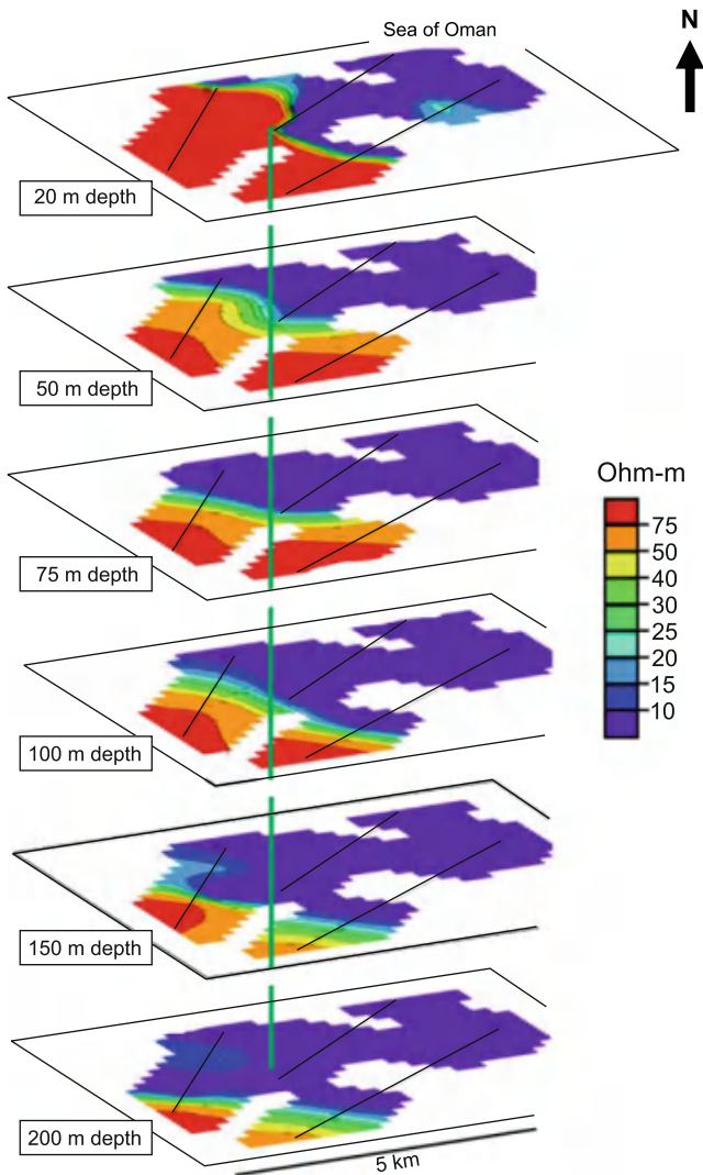
Fig. 11.5 TDEM-derived planar maps of formation resistivity at various depths at Wadi Al Hawasinah, Northern Oman. Low resistivities (blue shades) represent the presence of saline water, which progressively extend a greater distance landwards with depth (from Abdalla et al. 2010)
