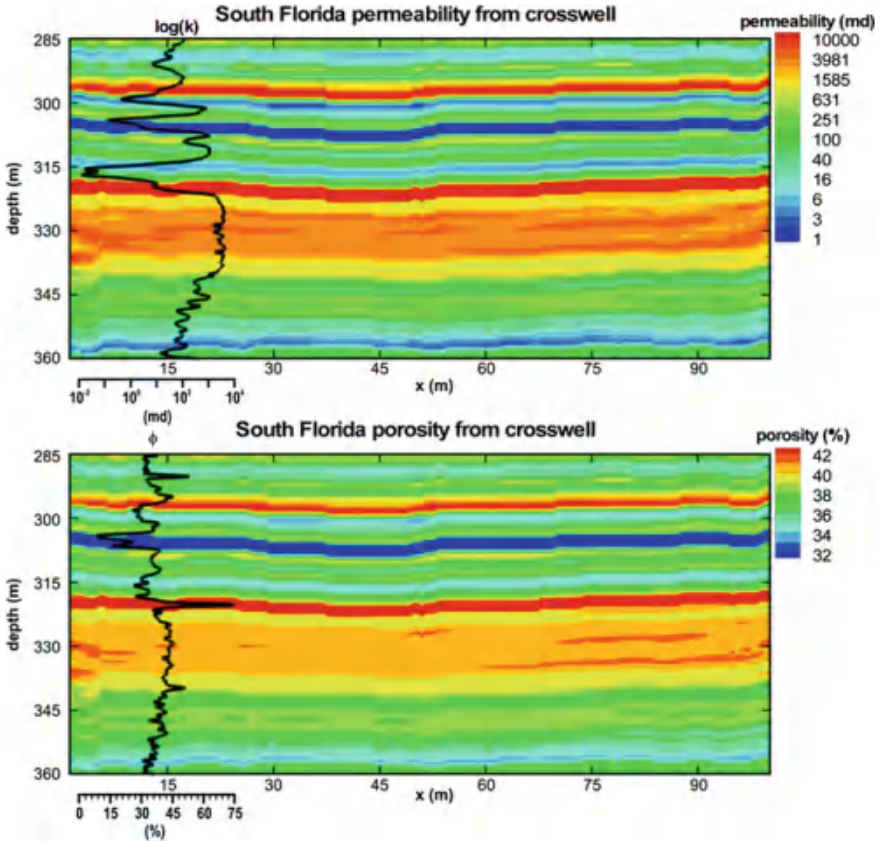
Fig. 15.1 Permeability image (top) and porosity image (bottom) computed from cross-well seismic data from the western Hillsborough aquifer storage and recovery system site, Palm Beach County, Florida. The respective well logs are superimposed on the images (from Parra et al. 2006)
