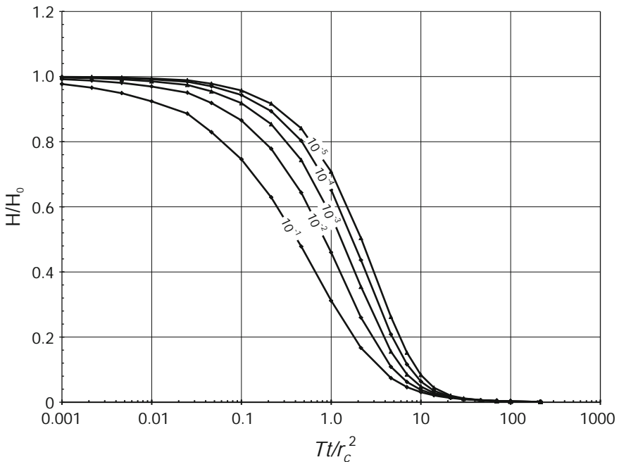
Fig. 8.7 Cooper et al. (1967) types curves for wells of finite diameter and a values of 10^{-1} , 10^{-2} , 10^{-3} , 10^{-4} , and 10^{-5}
