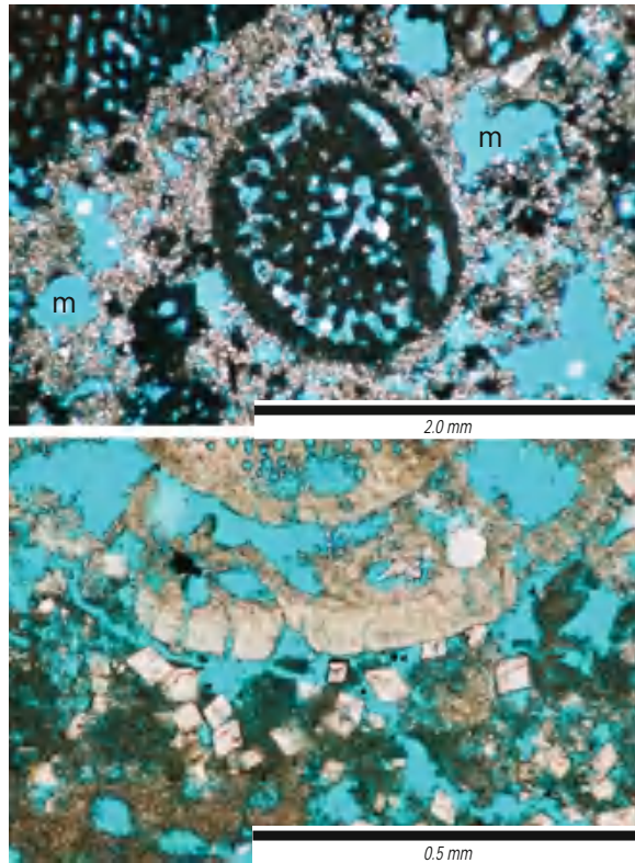
Fig. 9.4 Thin-section photomicrographs of dolomitic limestone from the Avon Park Formation (Middle Eocene), Daytona Beach, Florida. Porosity is filled with blue-dyed epoxy. Large foraminifera is evident in the middle of top photograph and top of the bottom photograph. Moldic pores (m) and dolomite crystals (clear rhombohedra) are evident
