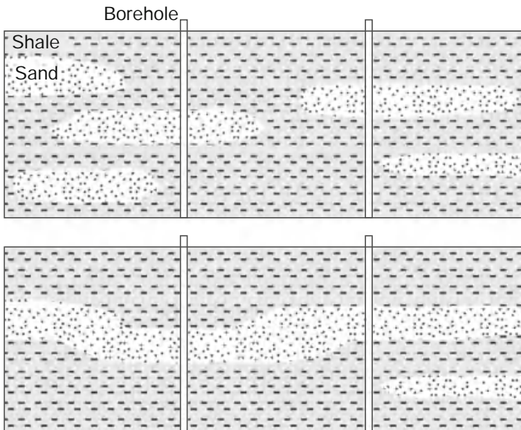
Fig. 16.4 Conceptual diagram of sand and shale systems with different degrees of connectivity of high-hydraulic conductivity sands. Aquifers with low connectivity of sand bodies (top) will have lower transmissivity than aquifers in which the sands are well connected (bottom). The degree of connectivity will not be evident in data from a small number of boreholes
