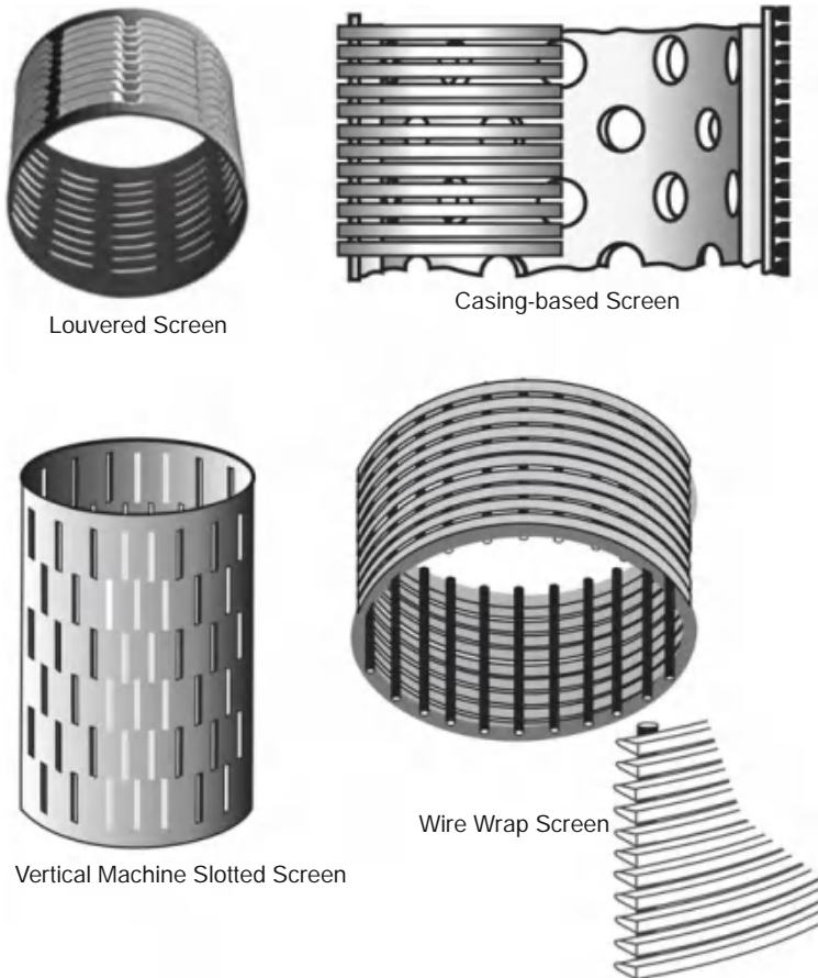
Fig. 6.13 Water well screen types (from Roscoe Moss 1990)
