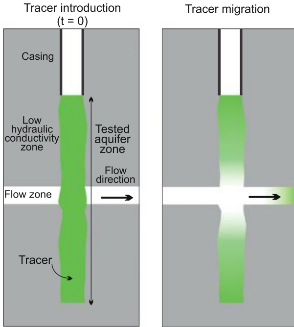
Fig. 13.8 Changes on the distribution of a tracer (green) released in a well for a natural or convergent forced-gradient test. a Tracer is introduced in manner so that the concentration in the well is near uniform in tested interval. b Tracer will preferentially enter a flow zone while remaining largely behind in depths of the borehole adjoining less conductive strata. The mass of tracer that reaches the pumped well or down-gradient production may be much less than would occur in a homogeneous aquifer in which all the tracer enters the tested interval
