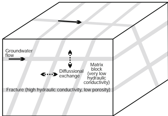
Fig. 17.3 Conceptual diagram of a dual-porosity system. Fractures (gray) have a relatively high-hydraulic conductivity but a very low porosity. The fracture-bound matrix blocks, in sedimentary aquifers, may have a low hydraulic conductivity but high porosity. The bulk of the groundwater flow occurs in the fractures but the most of water and solute storage occurs in the matrix
