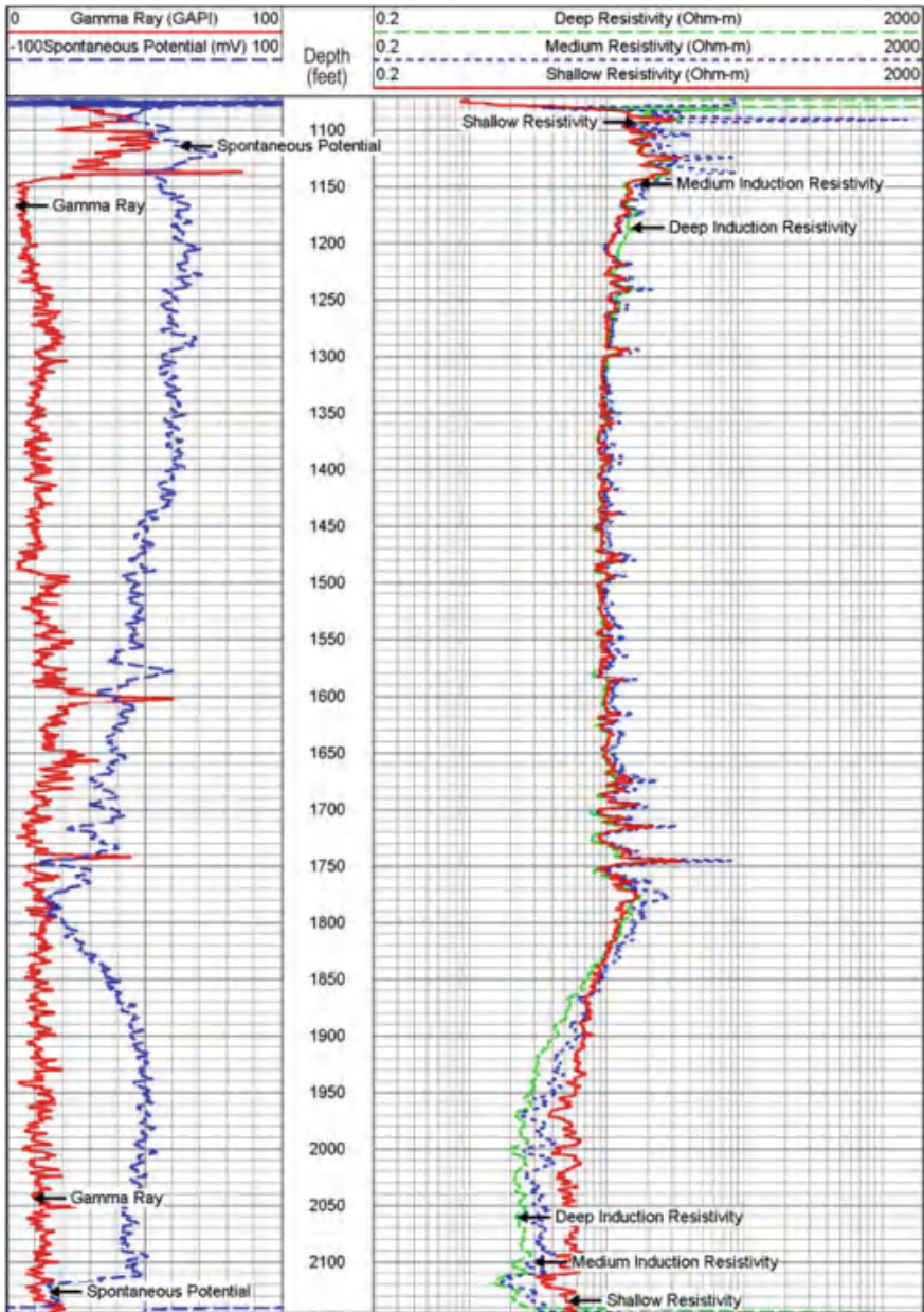
Fig. 10.4 Dual-induction log of a relatively homogenous limestone interval (Floridan Aquifer, Hiialeah, Florida). A pronounced down-hole increase in salinity from mildly brackish to seawater values is evident by the sharp decrease in resistivity from 1780 to 1950 ft. The increase in the difference in salinity between the drilling fluids and pore waters below 1780 ft allows for invasion to be detected as evidenced by separation of the resistivity tracks
