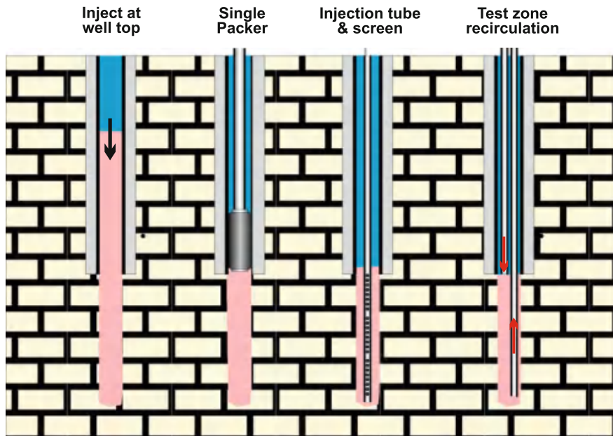
Fig. 13.7 Diagram of some tracer introduction options for a well. Tracer (pink) is poured into the well and then chased with clean water (blue). The volume of chase water can be reduced by setting a packer above the test interval and injecting the tracer through a smaller diameter tube. A more even tracer distribution in the tested interval may be achieved by injecting the tracer through a screen or perforated pipe. The top of the tested interval may be sealed off using a packer (not shown). An even tracer distribution may also be achieved by recirculating the tracer, which involves injection of the tracer at the top of the tested interval, while pumping water from the bottom of the interval at the same rate. The pumped water is reinjected into the well. A recirculation system could also be installed in an interval isolated by packers
