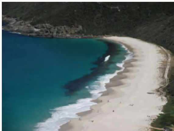
Fig. 3.21 Beach deposition between headlands, Western Australia near Albany
