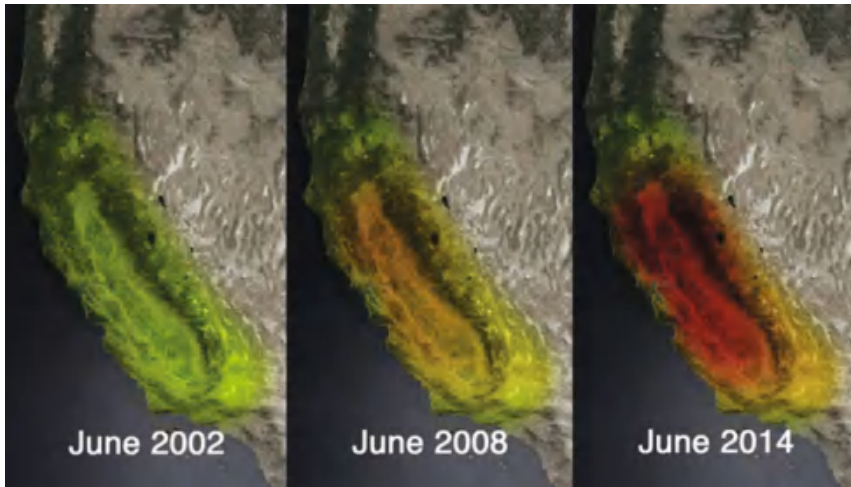
Fig. 11.15 GRACE images of declining water storage in California in June 2002 (left), June 2008 (center) and June 2014 (right). Colors progressing from green to orange to red represent greater accumulated water loss between April 2002 and June 2014 (from NASA/JPL-Caltech/University of California, Irvine)
