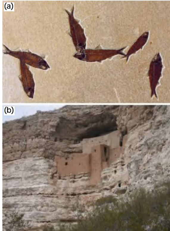
Fig. 3.18 a Fish fossils in the Eocene Green River Formation, Wyoming, USA (source U.S. National Park Service. b Ancient American Indian (Sinaguan) cliff dwelling constructed in the lacustrine Verde Formation, which contains both fine-grain limestone and siliciclastic deposits, Montezuma's Castle National Monument, Arizona, USA. Secondary porosity is well developed in the limestone strata
