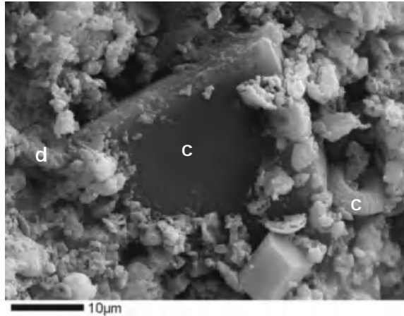
Fig. 9.5 SEM photograph of a sample of the Avon Park Formation (Middle Eocene), Daytona Beach, Florida, showing smooth-faced, euhedral dolomite crystal (d) and microporous matrix. Microfossils (coccoliths; c) are evident
