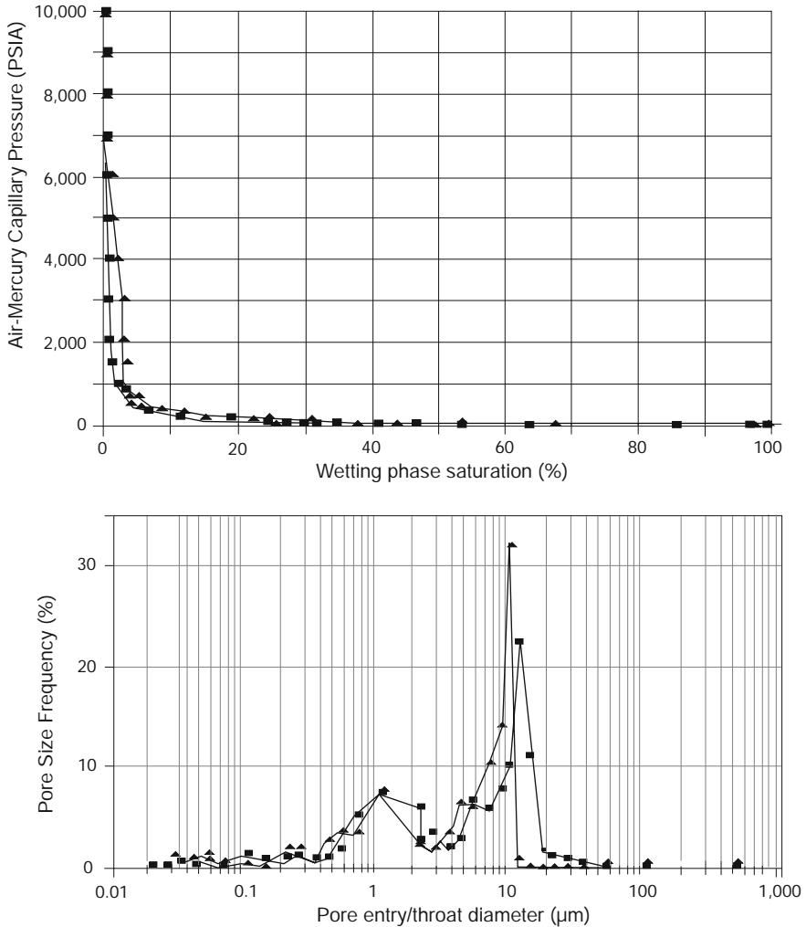
Fig. 9.2 Example of mercury-injection porosimetry data. Plots are of capillary pressure versus saturation (top) and pore throat diameter distribution (bottom) under ambient (squares) and in situ stress (triangles) conditions (from Keighin 1997)
