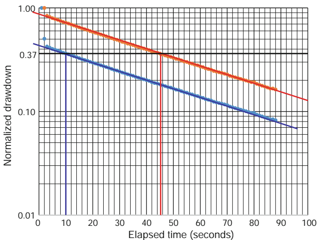
Fig. 8.4 Example of potential error in the application of Hvorslev method from the use of an incorrect initial head value ( H_0 ) from ‘splash’ or other effects. Use of an anomalous initial head increase of 1.67 m at t = 1 s gives a basic time lag ( T_0 ) of 10 s (blue values) compared to value of about 45 s obtained if the increase of 0.84 m at t = 2 s is used (red values). The 0.84 m rise in water level is consistent with the slug volume
