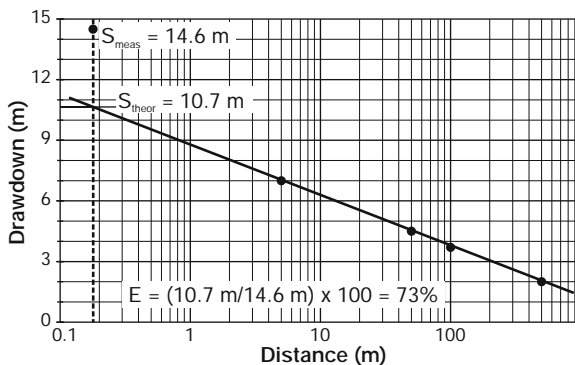
Fig. 6.2 Well efficiency can be determined from the ratio of measured drawdown in a well ( S_{\text{meas}} ) to the theoretical drawdown ( S_{\text{theor}} ) obtained by extrapolating the distance-drawdown data to the well radius
