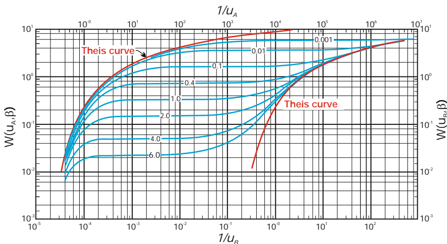
Fig. 7.8 Neuman (1975) delayed-yield type curves, which consists of early and late Theis curves (red) and a series of b curves (blue)
