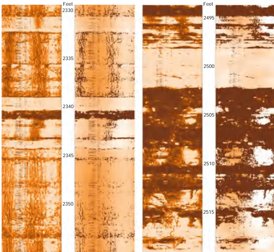
Fig. 10.13 Acoustic televiewer images of horizontally bedded limestone and dolomite (left) and fractured, vuggy dolomite (right), Eocene-aged Avon Park Formation, Hialeah, Florida. Low-porosity, hard dolomite is light colored, porous limestone appears orange-brown, and open pores are very dark colored
