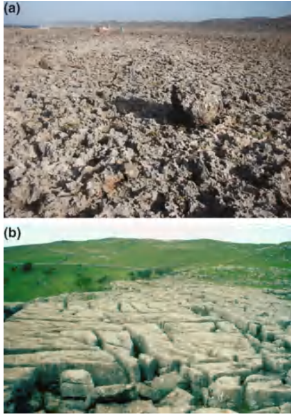
Fig. 18.2 Examples of karren landforms. a Sharp-edged phytokarst common along parts of the coast of Aruba. b Clints (flat-topped slabs) and grikes (solution-widened fissures) in Carboniferous limestones in the Yorkshire Dales, near Malham, England (bottom)
