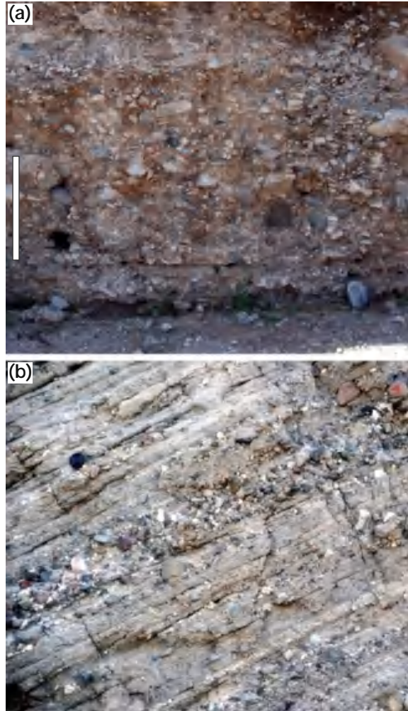
Fig. 3.11 Alluvial-fan sediments. a Proximal fan coarse debris-flow deposit, White Tank Mountain Park, near Phoenix, Arizona (scale is approximately 1 m). b Sandy alluvial-fan deposits, Death Valley National Park, California (lens cap for scale)
