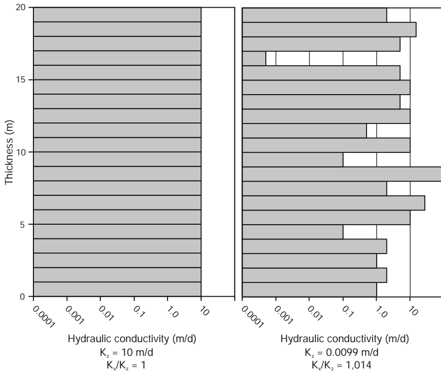
Fig. 1.5 Conceptual diagram comparing the equivalent vertical hydraulic conductivity ( K_z ) and anisotropy ratio ( K_x/K_z ) of a hypothetical homogeneous aquifer (left) and layered heterogeneous aquifer (right) that have the same transmissivity and average horizontal hydraulic conductivity
