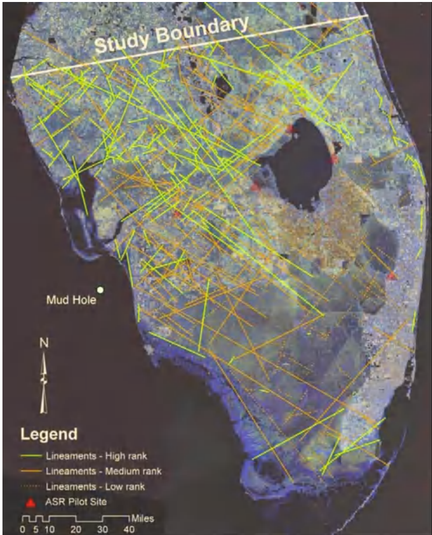
Fig. 17.6 Map showing lineaments identified in south Florida on a Landsat mosaic (Fies 2004)
