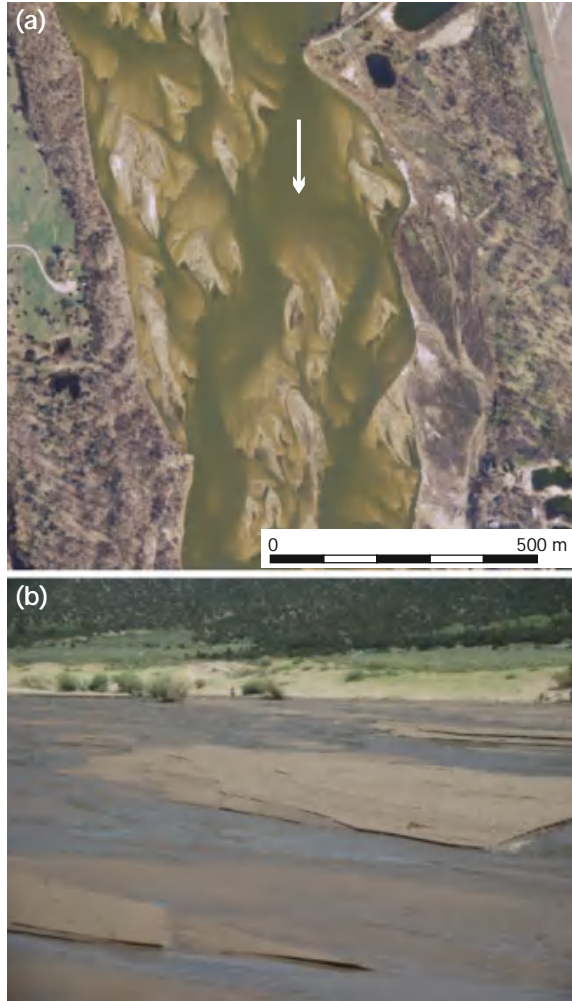
Fig. 3.8 a Aerial photograph of the braided Platte River near Omaha, Nebraska, USA. Flow direction (arrow) is to the south (source U.S. Geological Survey). b Shallow braided stream at Great Sand Dunes National Monument, Colorado, USA (note people on far bank for scale)
