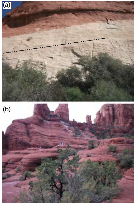
Fig. 3.17 a Massive eolian sandstones (Jurassic), Red Rock Canyon, near Las Vegas, Nevada, USA. Boundary between large cross-bedding sets is evident (dashed line). b Massive eolian sandstones (Permian), Sedona, Arizona, USA (note people for scale)
