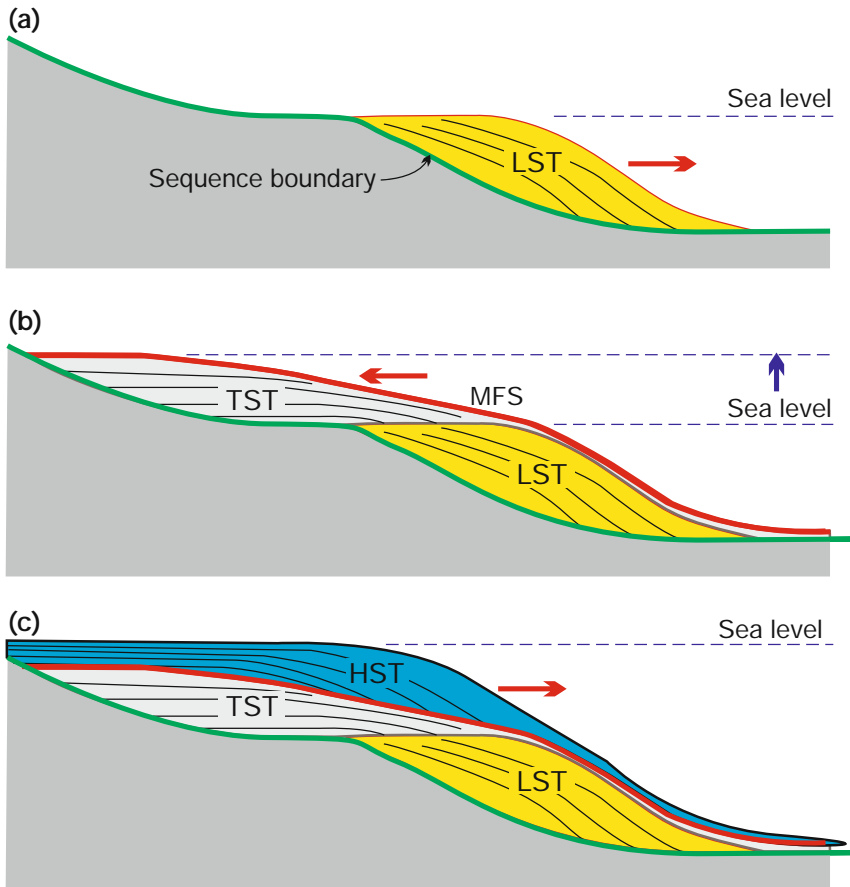
Fig. 2.3 Basic sequence stratigraphy diagram. a Lowstand system tract (LST) offlaps on the sequence boundary. b Transgressive system tract (TST) overlies the sequence boundary. Its upper boundary is the maximum flooding surface (MFS), which is the surface of deposition at its maximum landward position (i.e., time of maximum transgression). c Highstand systems tract (HST) marks return of progradation with the offlap of strata on the MFS
