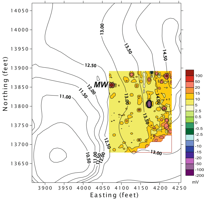
Fig. 11.3 EM survey data from the USEPA characterization test cell (CTC) site at the Naval Base Ventura County, Port Hueneme, California. Detected anomalies were ferrous and nonferrous metallic objects within the depth range of the instrument, including a monitoring well (MW). Ground elevation contours are in feet (from Werkema 2004)
